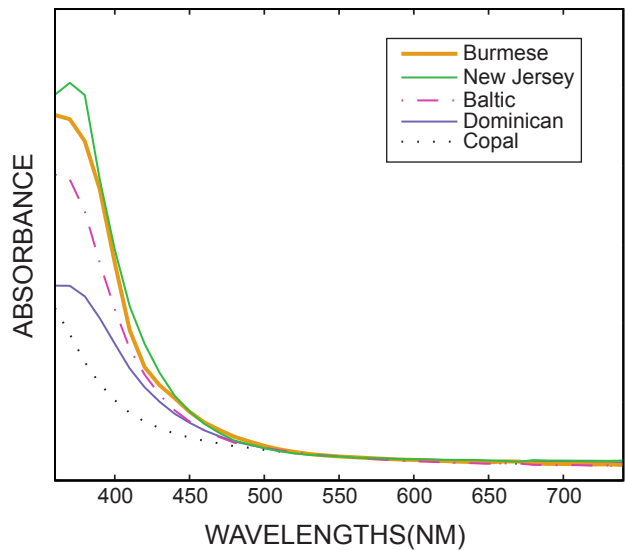
FIGURE 5. Distinct absorbance spectra (averaged) for each of the five fossil resins before aging.
